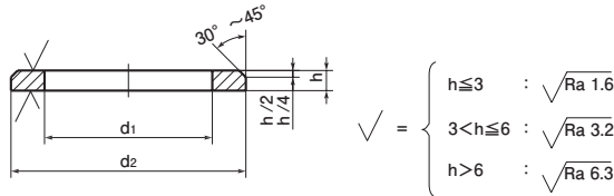
Standard-sized chamfering - Shape of part grade A
